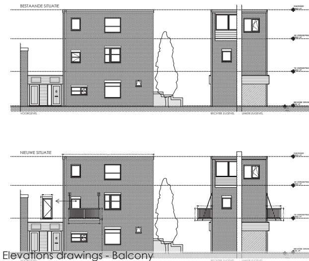
Elevations drawings - Balcony
