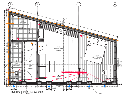
Layout plan - Small apartment
