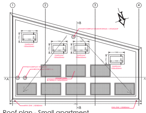
Roof plan - Small apartment
