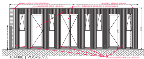
Elevations - Small apartment
