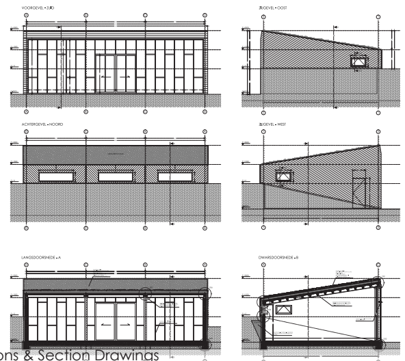
Elevations & Section Drawings
