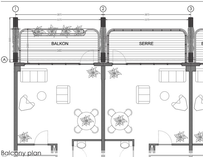
Balcony plan
