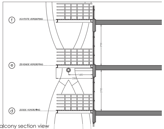
Balcony section view
